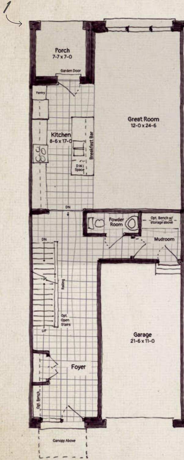
MAIN FLOOR
